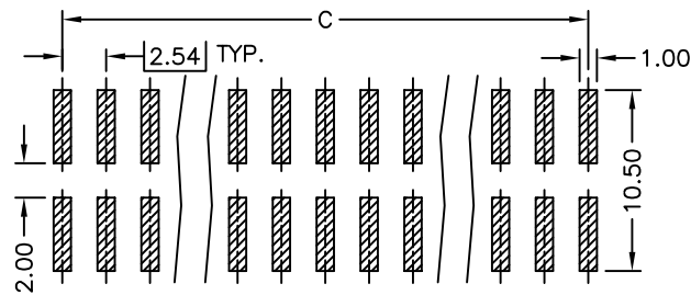
RECOMMEND P.C.B. LAYOUT TOP VIEW
