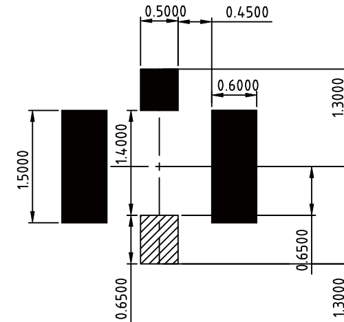
■ GROUND PAD RECOMMENDED PCB LAYOUT
