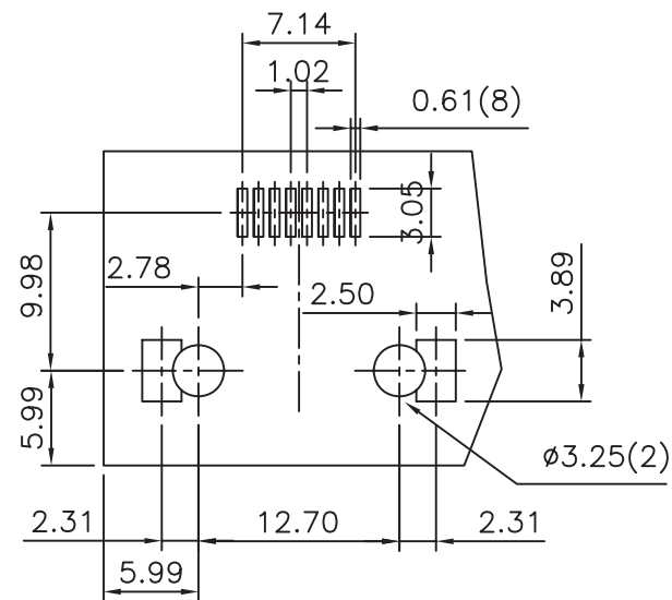
PCB LAYOUT
