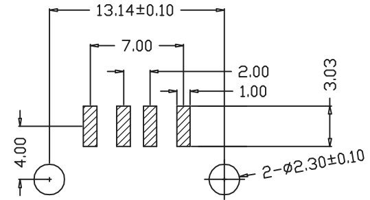
RECOMMENDED P.C.B. PATTERN LAYOUT
