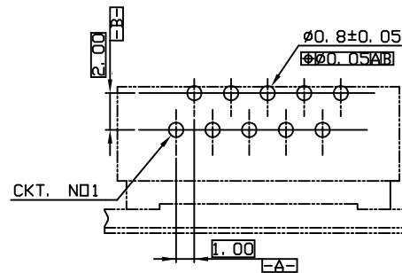
PC BOARD LAYOUT: COMPONENT SIDE PCB T=1.6mm
