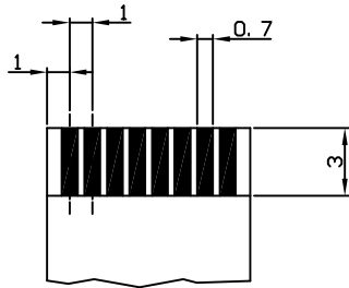
FFC/FPC DIMENSION THICKNESS 0.3±0.05mm TOLERANCE: 0.05mm
