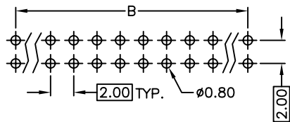
RECOMMEND P.C.B. LAYOUT BOTTOM VIEW
