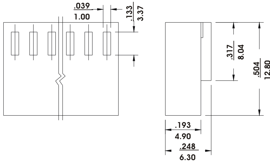
Dimension information-inch/mm
