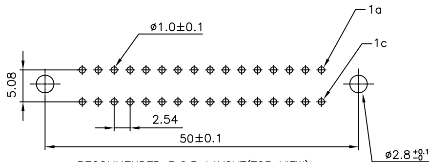
RECOMMENDED P.C.B LAYOUT(TOP VIEW) TOLERANCES: ±0.10mm
