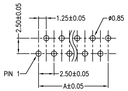
STANDARD PCB LAYOUT
