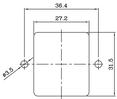
PANEL CUT-OUT
