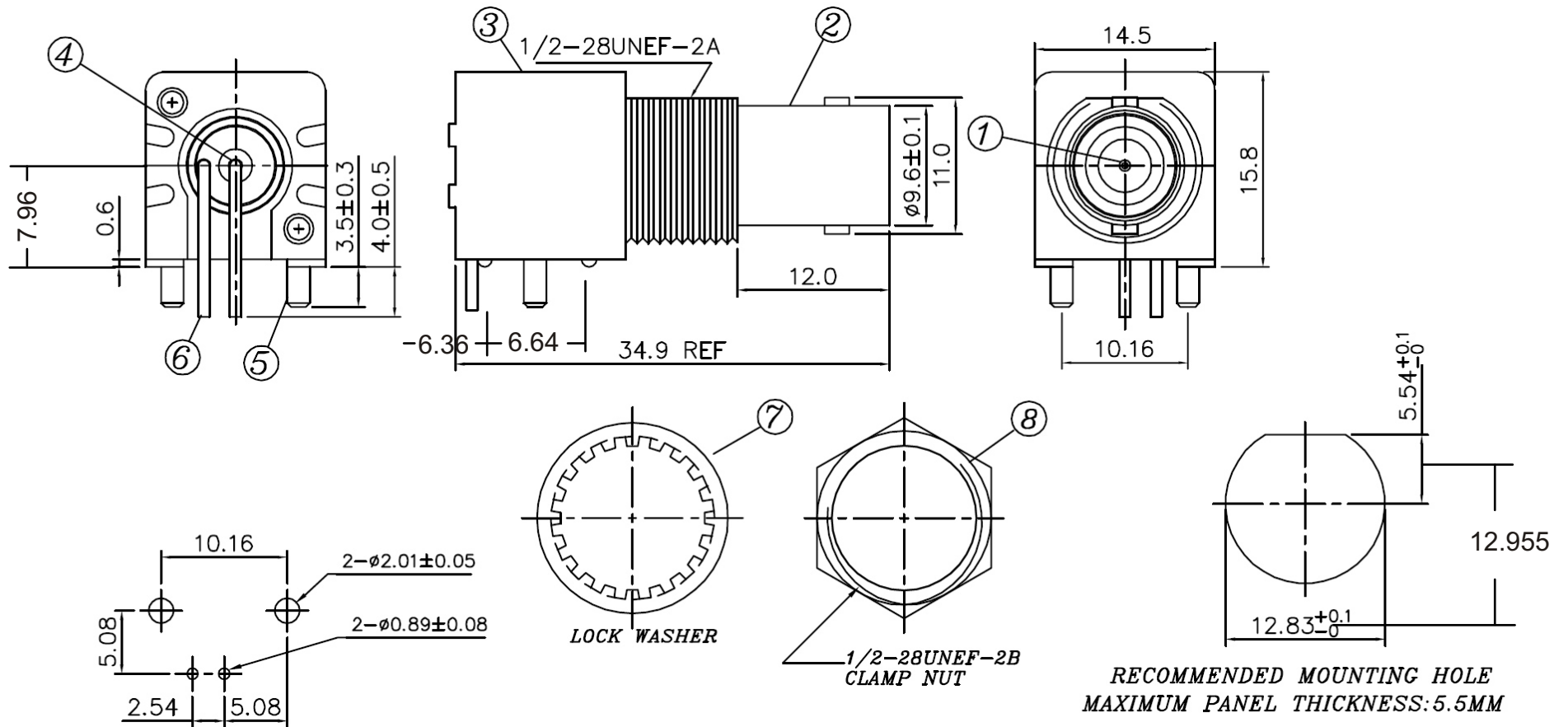
RECOMMENDED PC BOARD LAYOUT WITHOUT MOUNTING POSTS
