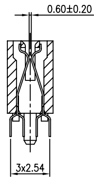
PLASTIC POST
