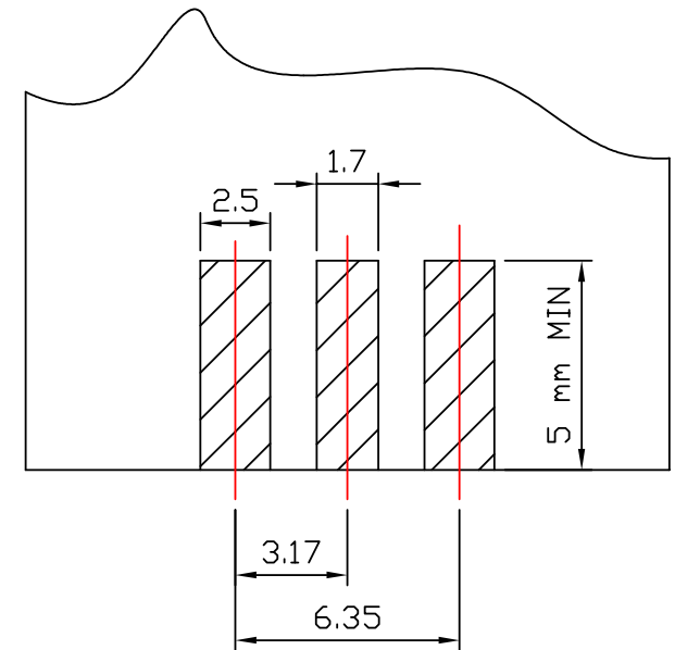
LANDING PAD DIMENSIONS
