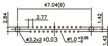
Recomended PCB Layout
