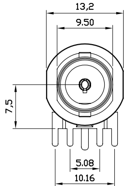
PANEL LAYOUT
