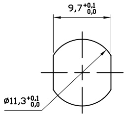
PANEL LAYOUT
