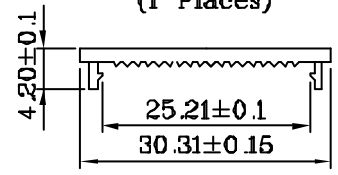
Termination Cover (1 Places)
