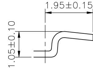
SEC:C-C
