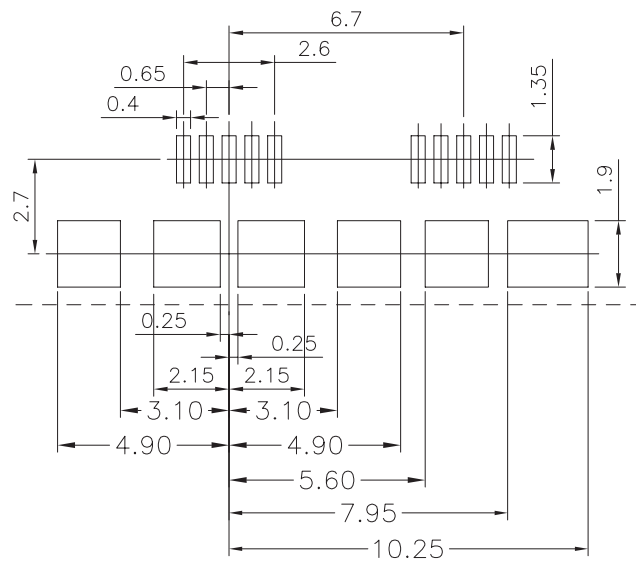
P.B.C LAYOUT TOP VIEW ±0.05
