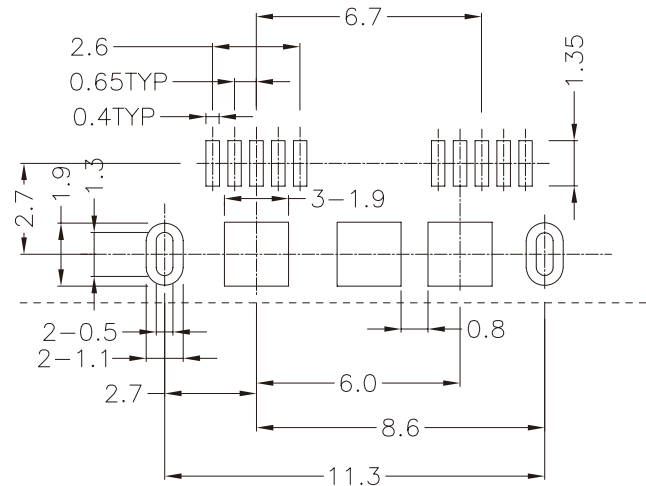
P.B.C LAYOUT TOP VIEW ±0.05
