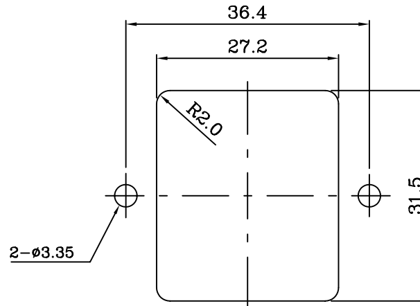
PANEL CUT-OUT
