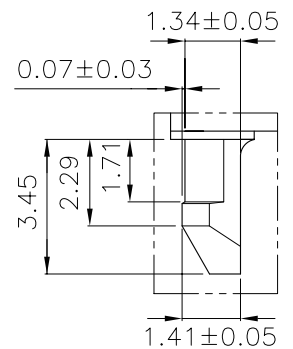
DETAIL X
