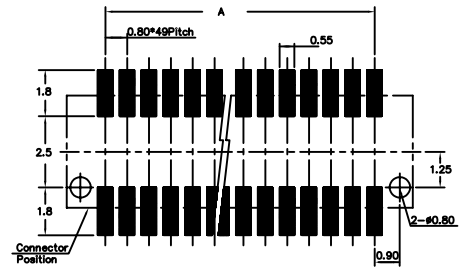
PCB Layout For Surface Mounting
