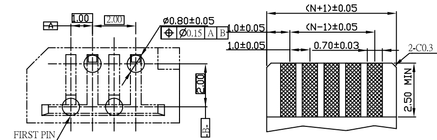
FPC THICKNESS=0.30mm TOLERANCE:0.05mm
