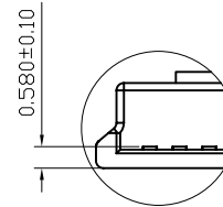
VIEW A 5:1
