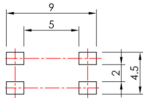
P.C BOARD MOUNTING HOLE DIMENSIONS
