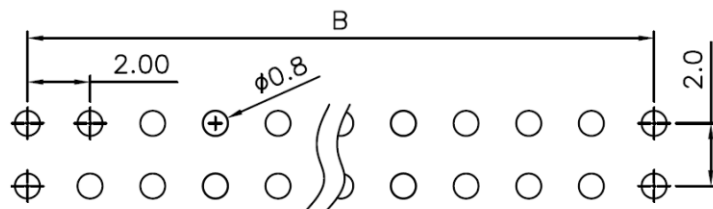
P.C. Board Layout (Tolerance: ±0.05)
