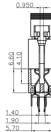
SECTION:A-A SCALE:2/1
