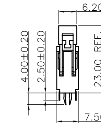
SECTION:A-A SCALE:2/1
