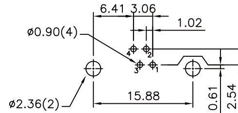
PCB LAYOUT Ref.
