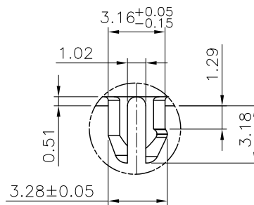
DETAIL Z SCALE 2:1
