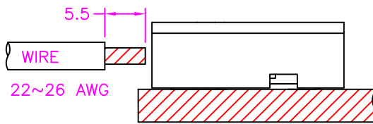
ASSEMBLY
