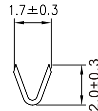
B-B SECTION
