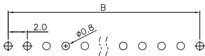
P.C. Board Layout (Tolerance: ±0.05)
