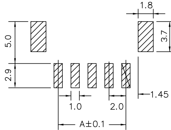
RECOMMENDED P.C. BOARD LAYOUT DIMM.
