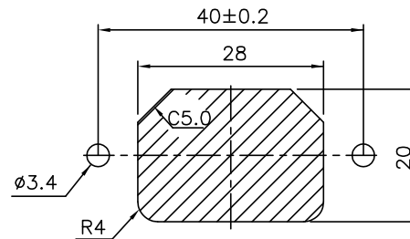
Mounting inlet flange in front of cover.
