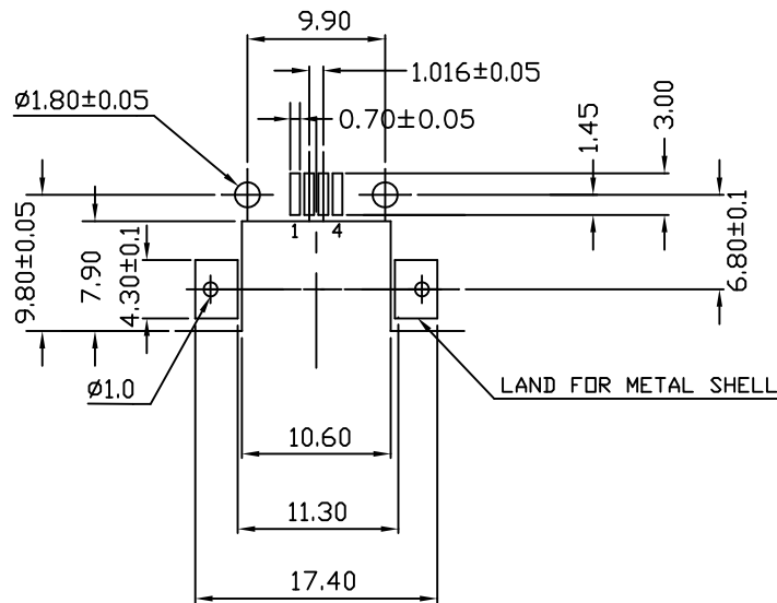
PCB LAYOUT
