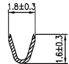
B-B SECTION
