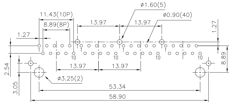
PCB LAYOUT Ref.
