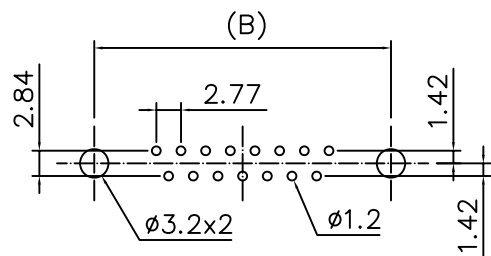
Recomended PCB Layout
