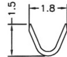
B-B SECTION
