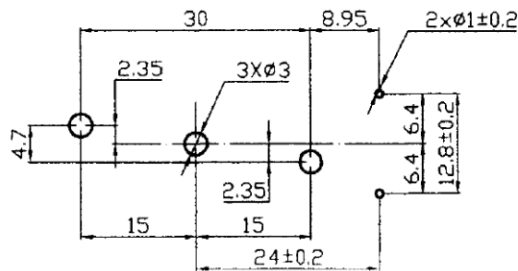
PCB/MOUNTING LAYOUT
