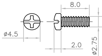
SCREW A TYPE FOR LOCK INSULATOR (4 PCS)
