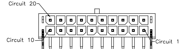
20PIN
