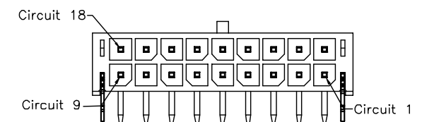
18PIN
