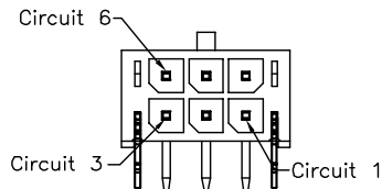
6PIN
