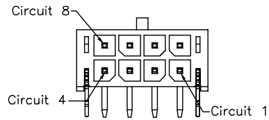
8PIN
