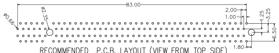
RECOMMENDED P.C.B. LAYOUT (VIEW FROM TOP SIDE)
