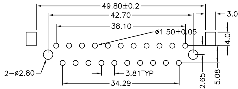
PCB LAYOUT
