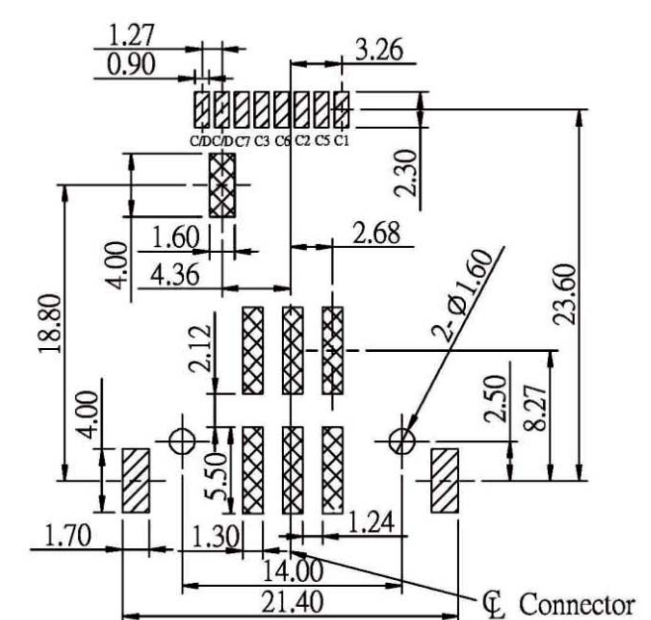
PCB LAYOUT
