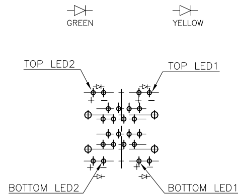
LED SCHEMATIC
