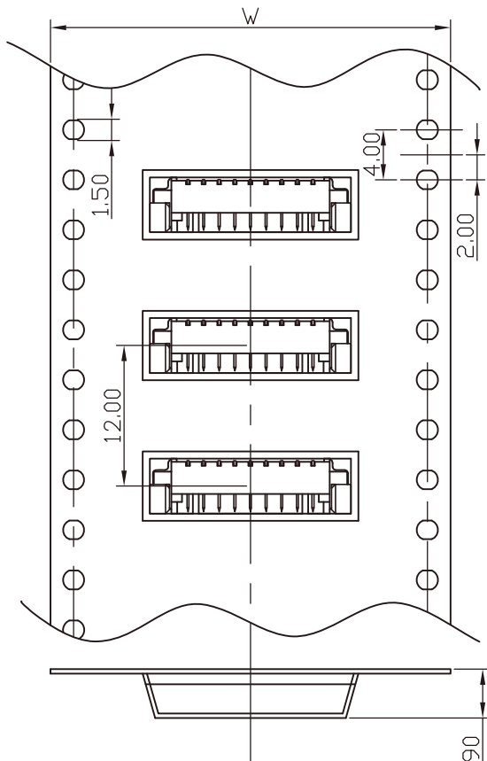
CARRIER FOR 10 TO 15PIN
