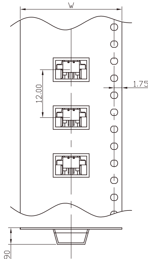
CARRIER FOR 2 TO 9PIN
