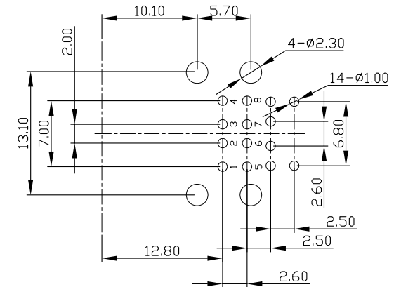
P.C.B LAYOUT BOTTOM VIEW P.C.B Tolerance ±0.1
