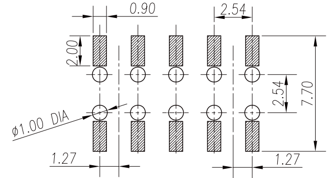
RECOMMENDED P.C.B LAYOUT FOR TOP ENTRY
