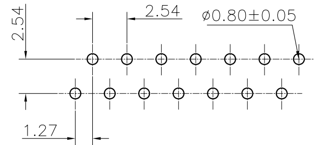
PCB Layout
